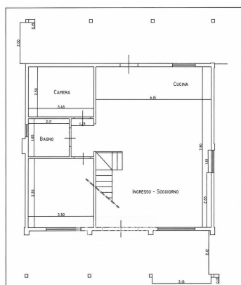
PIANO TERRA
